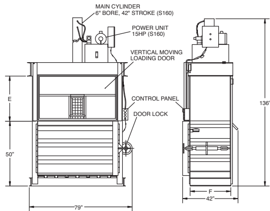
Standard 60" Baler
